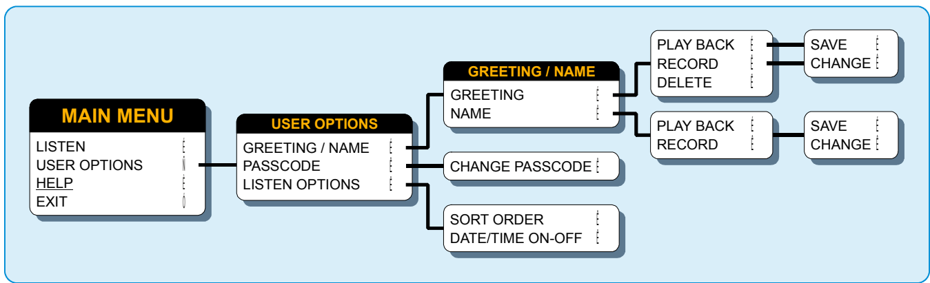
Figure 2: Customizing your Mailbox
