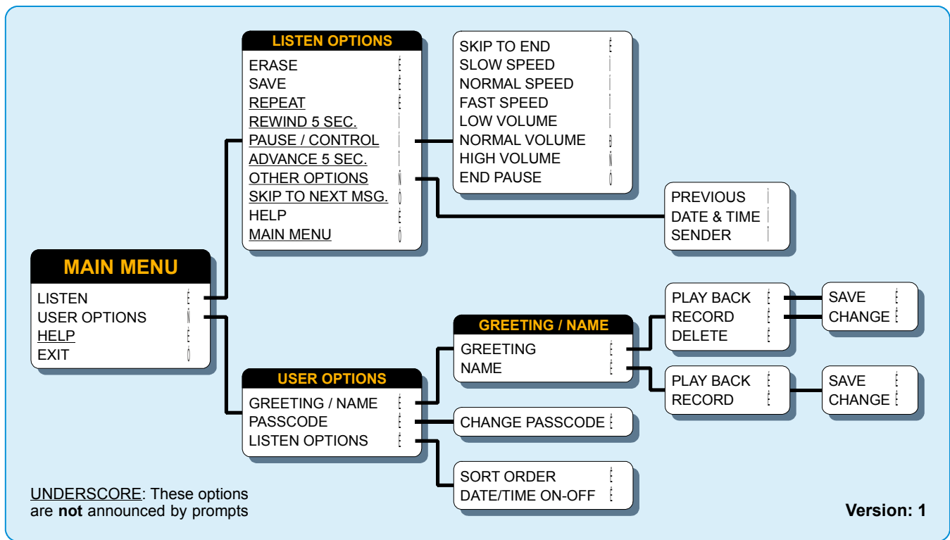
Figure 1: Complete babyMAIL Roadmap
